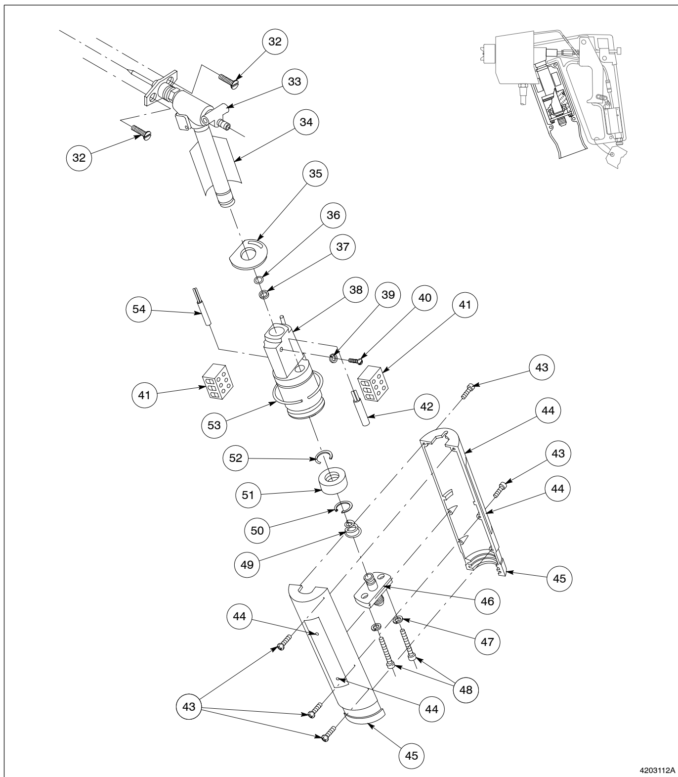
Fig. 8-2 AD-31 Spray Handgun - Pivot Sleeve Section (RTD-Style), Models SC, ST, and STL
