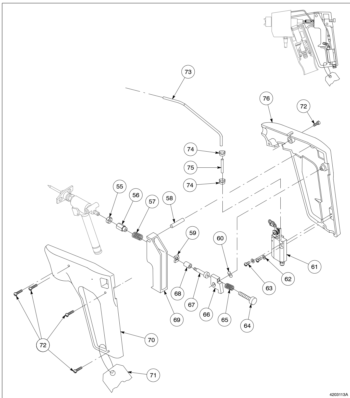
Fig. 8-3 AD-31 Spray Handgun - Trigger Section (RTD-Style), Models SC, ST, and STL
