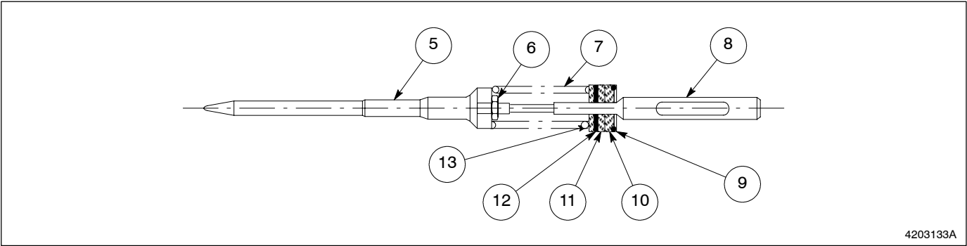
Fig. 8-9 Packing Cartridge Assembly
