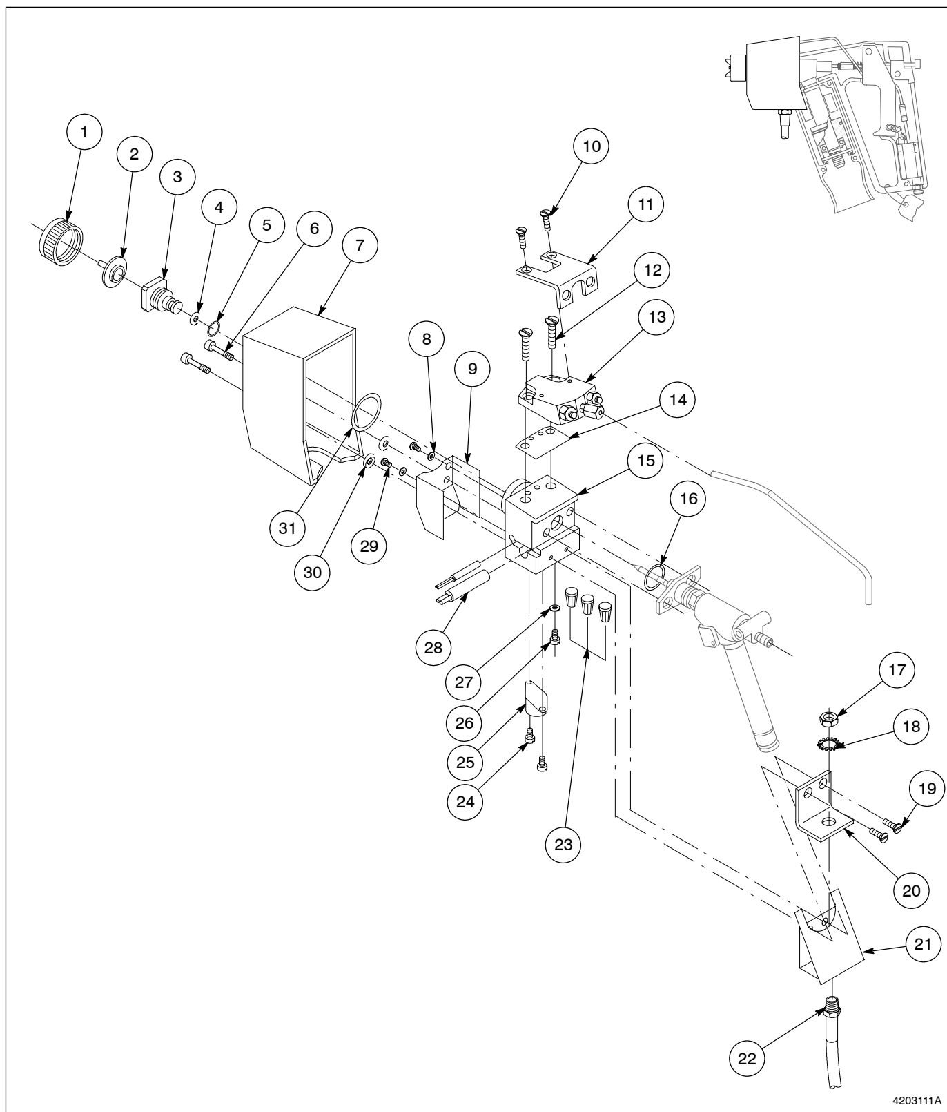
Fig. 8-1 AD-31 Spray Handgun - Nozzle Section (RTD-Style), Models SC, ST, and STL
