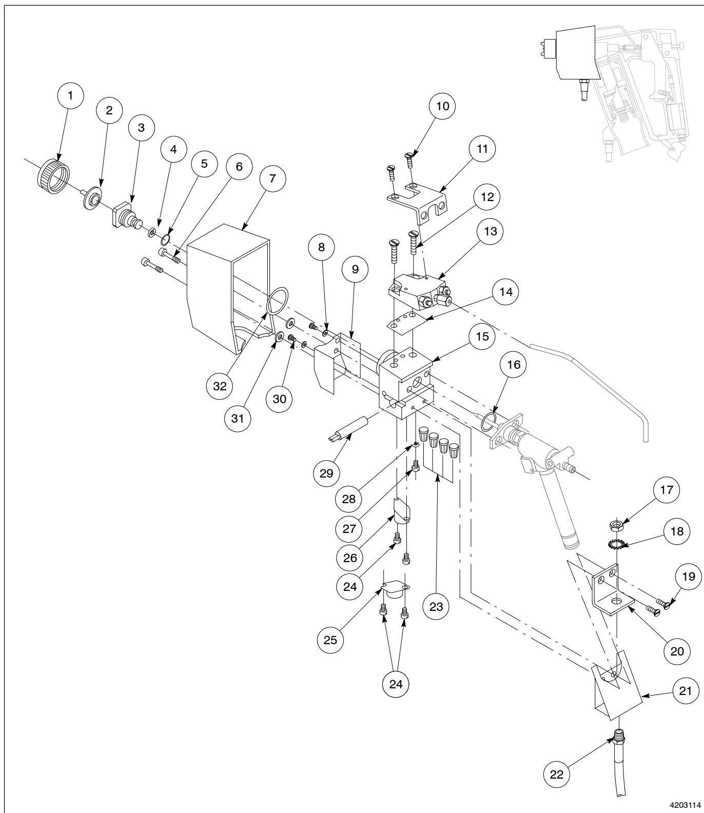
Fig. 8-4 AD-31 Spray Handgun - Nozzle Section (Thermostat Style), Models SA, SD, SDL, SE
