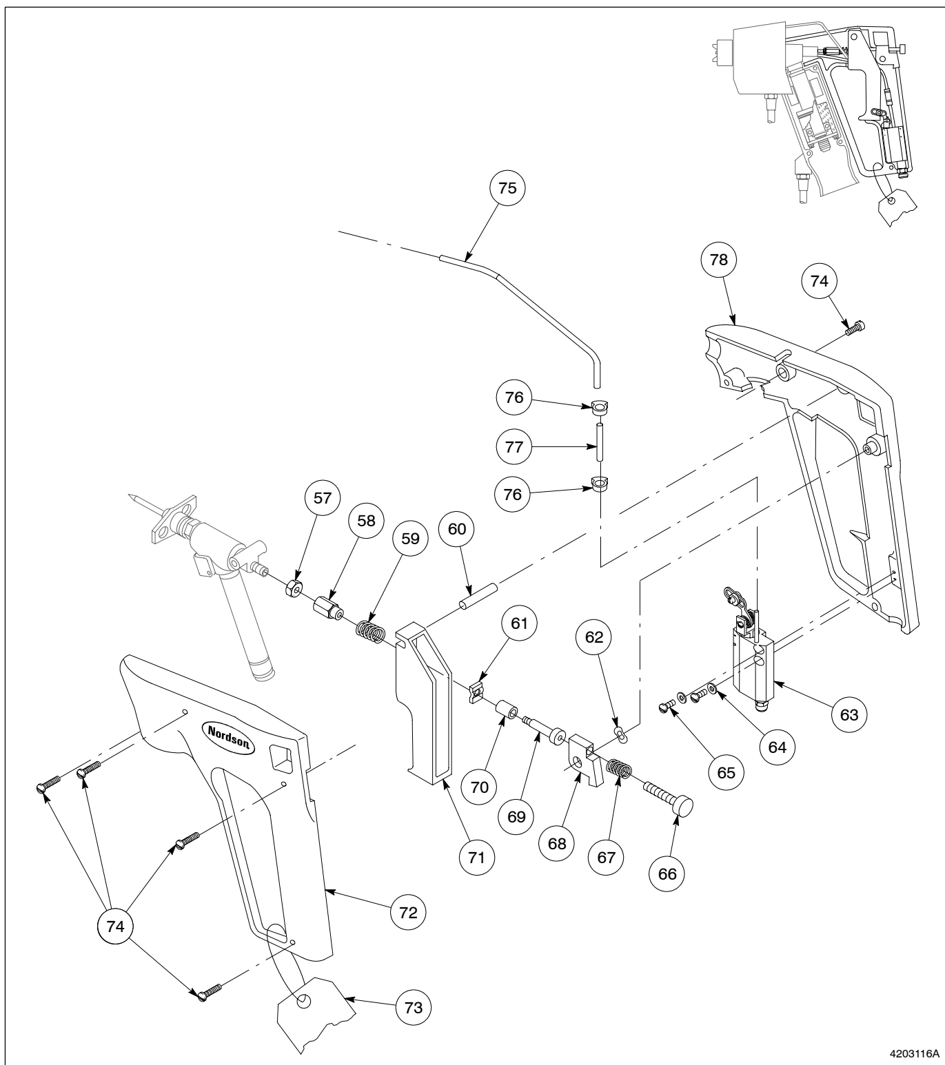
Fig. 8-6 AD-31 Spray Handgun - Trigger Section (Thermostat Style), Models SA, SD, SDL, SE
