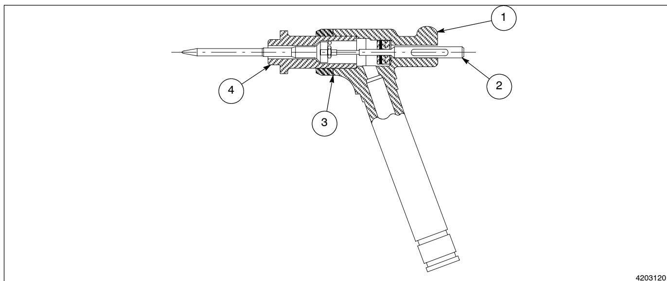
Fig. 8-8 Gun Body Assembly
