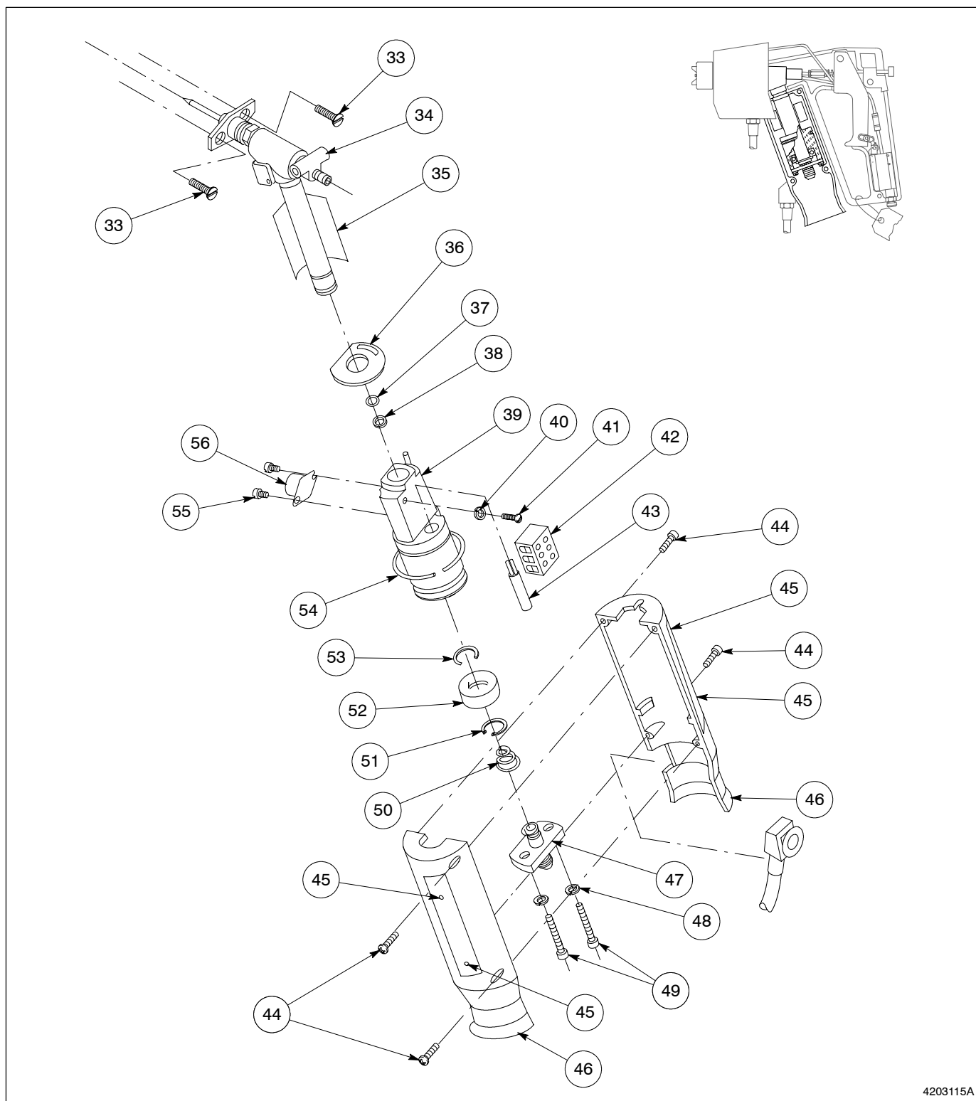
Fig. 8-5 AD-31 Spray Handgun - Pivot Sleeve Section (Thermostat Style), Models SA, SD, SDL, SE
