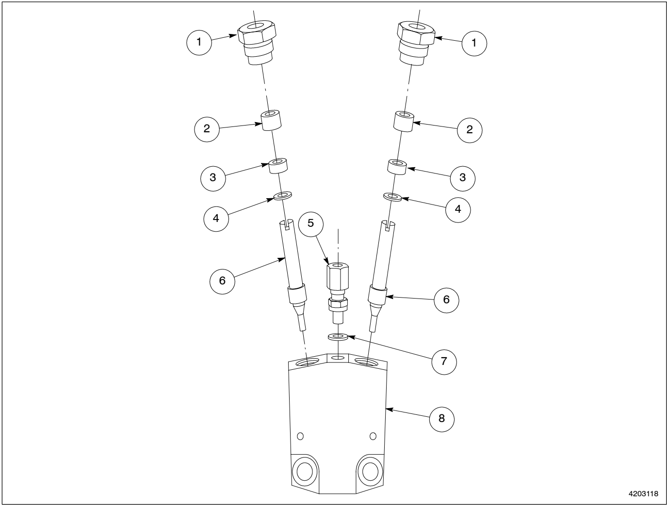
Fig. 8-7 Dual Valve Assembly
